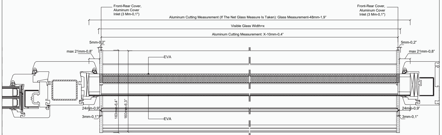
Fig: Horizontal Sercair System Detail - Frame / Sash Profile (Triple Glazing)-S2 Section
