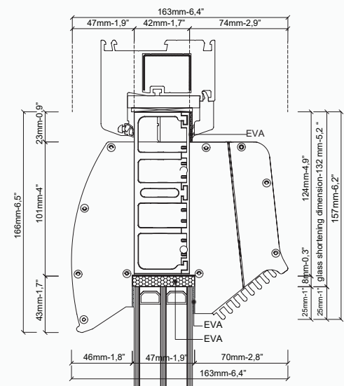
Fig: Frame / Sash Profile (Triple Glazing)
